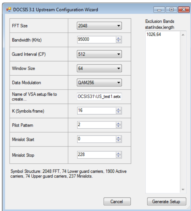
Figure 10 DOCSIS 3.1 Upstream
